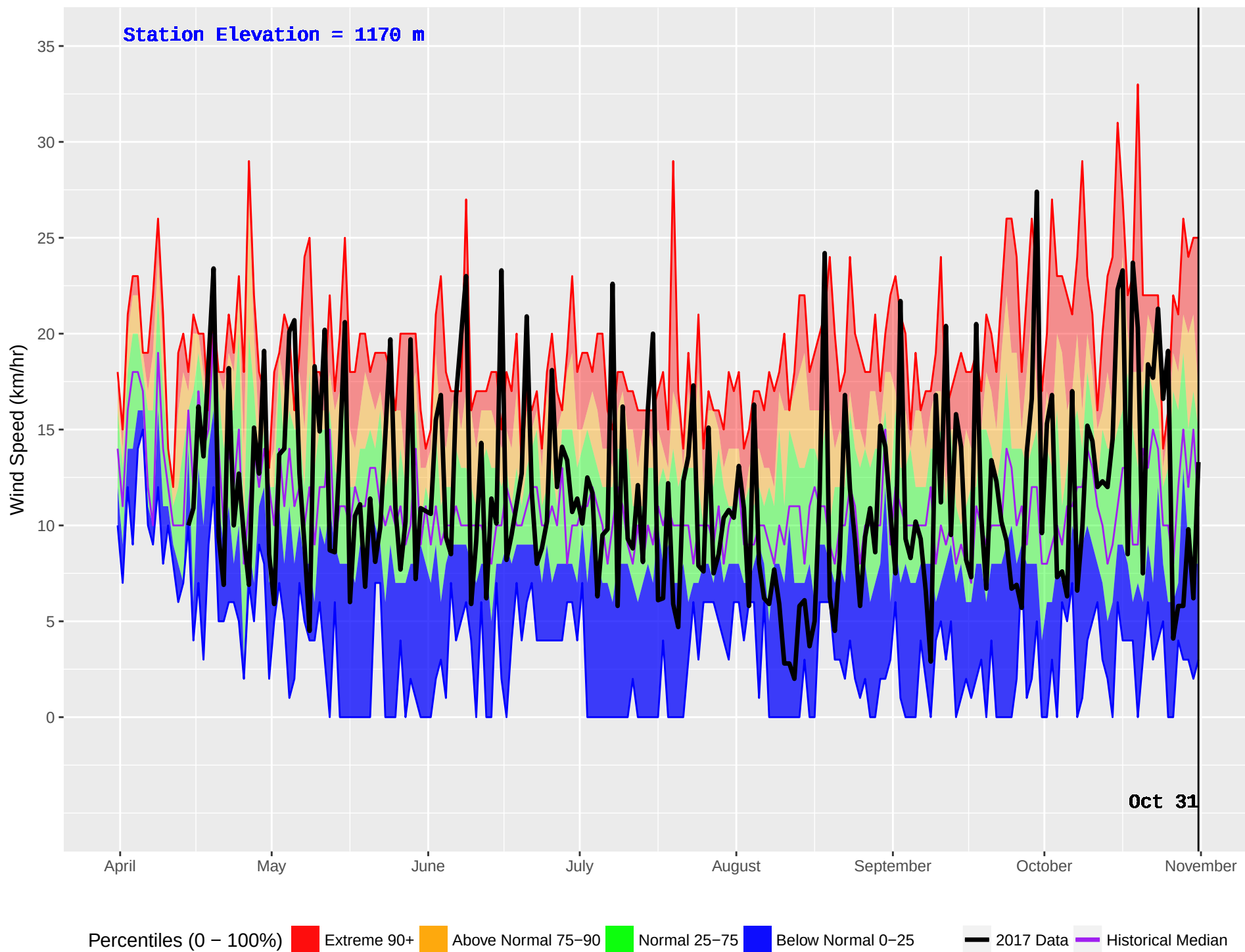
YOUNG LAKE (235) : Historical (2001–2016) and Current (2017) Noon Wind Speed
