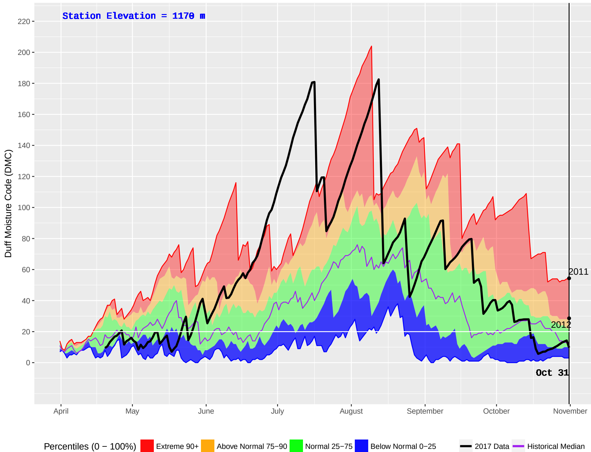
YOUNG LAKE (235) : Historical (2001–2016) and Current (2017) Noon Duff Moisture Code (DMC)
